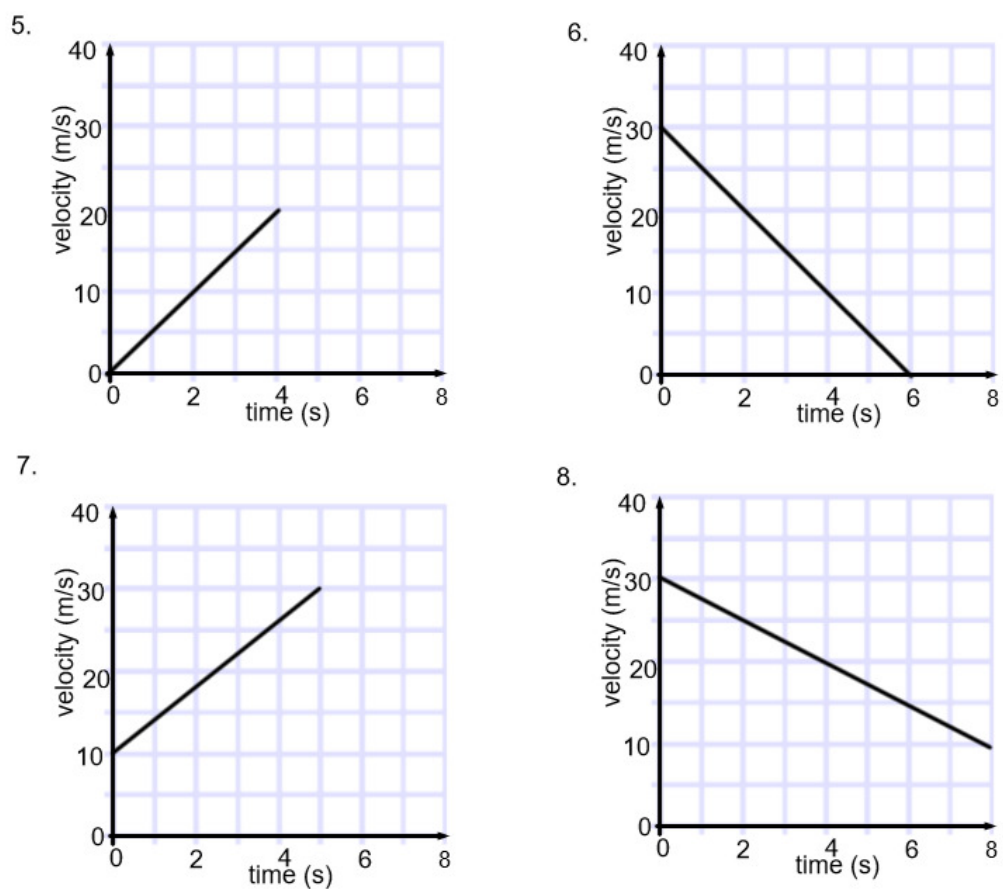
Fig 6.4 - Graphs 5-8: find the acceleration of each object (Questions 9-12)
