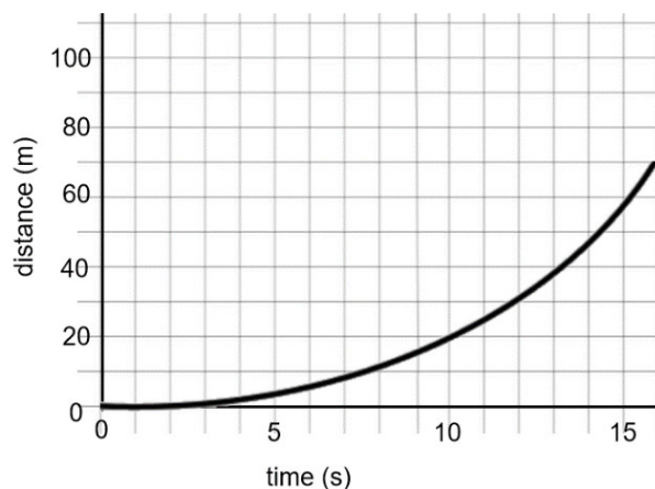
Fig 5.5 - Positive acceleration: curve becomes steeper over time
