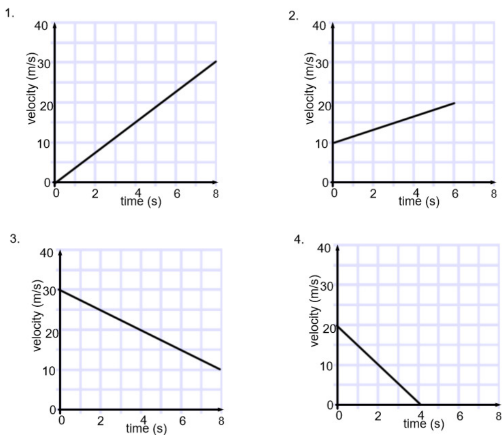
Fig 6.3 - Graphs 1-4: find the acceleration of each object (Questions 5-8)
